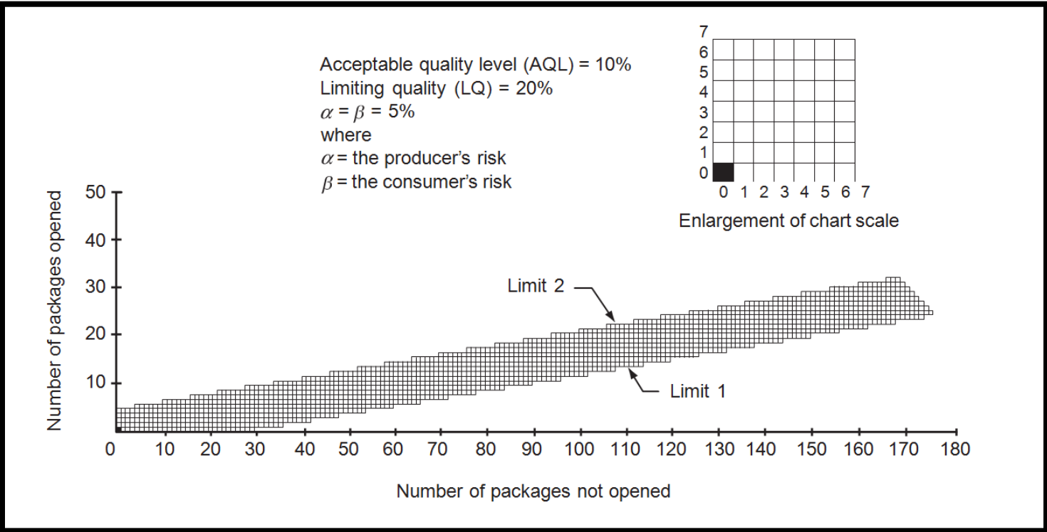
Figure 2. Chart of a sequential child-resistant effectiveness test procedure (without demonstration) for reclosable child-resistant packages
